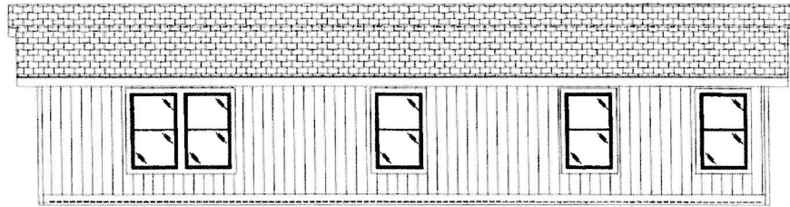
REAR SIDEWALL
